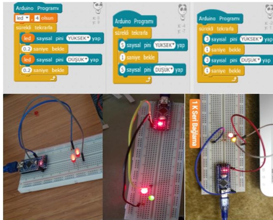
Figure 1. LED Brightness in a Series Circuit with a one k \Omega Resistor
